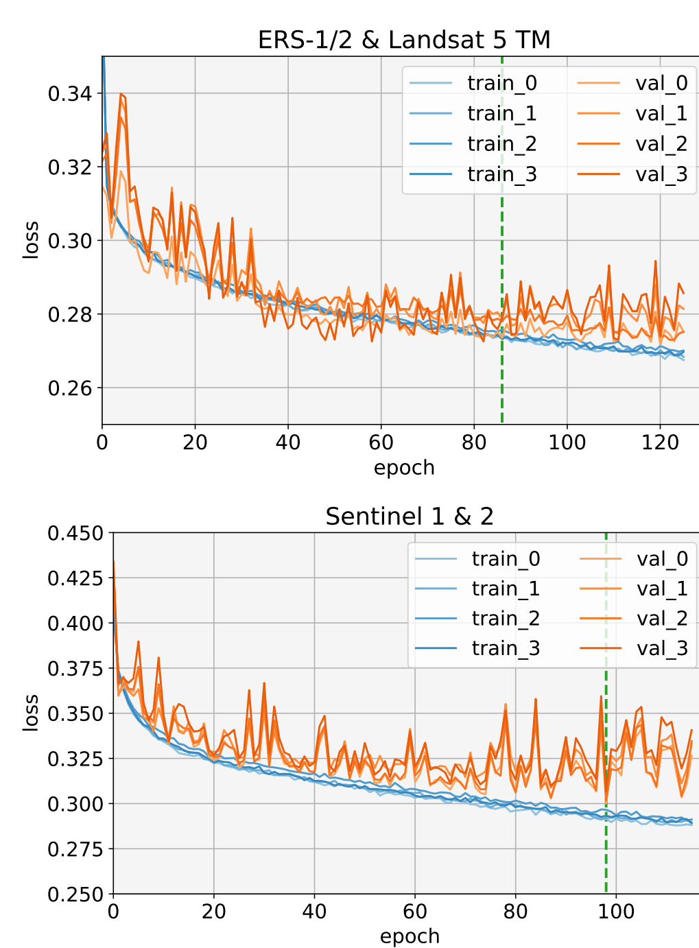
Figure 4. Loss values over epochs for both eras for the ensemble with both multispectral optical and SAR data. The green vertical indicates the best ensemble parameters for each era.
