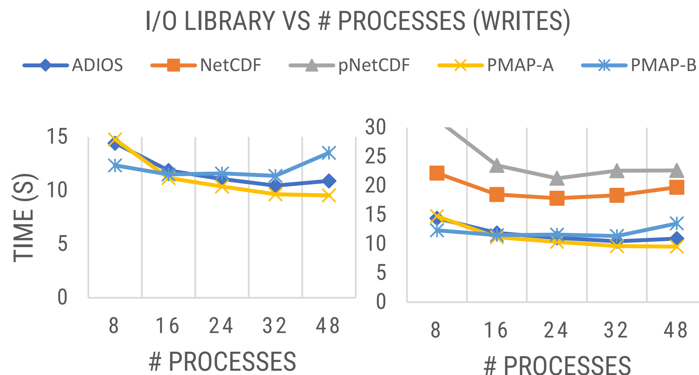
Figure 3: Writes
