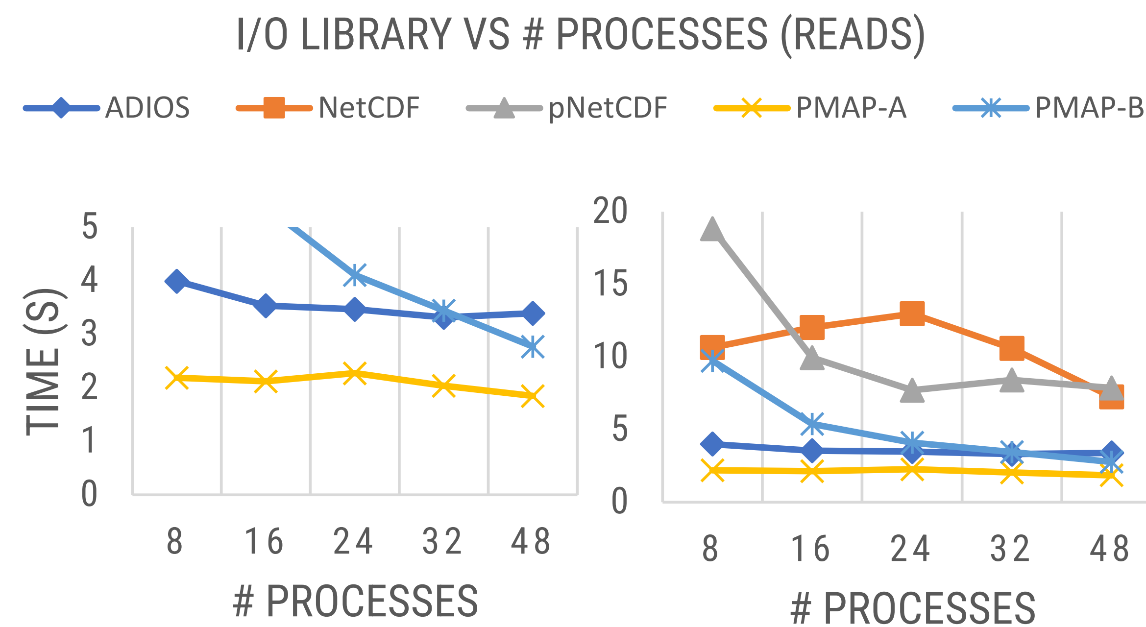
Figure 5: Reads
