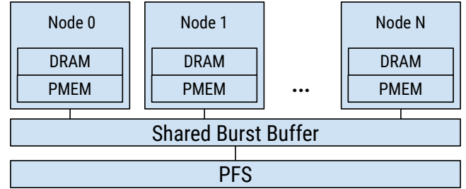
Figure 1: Basic Machine Architecture
